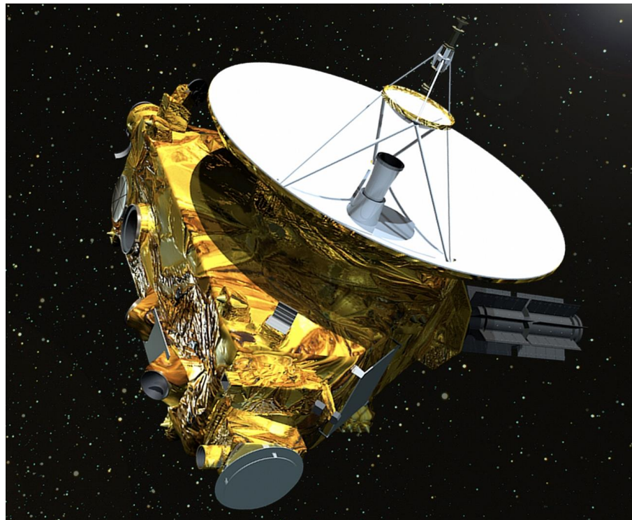
New Horizons
