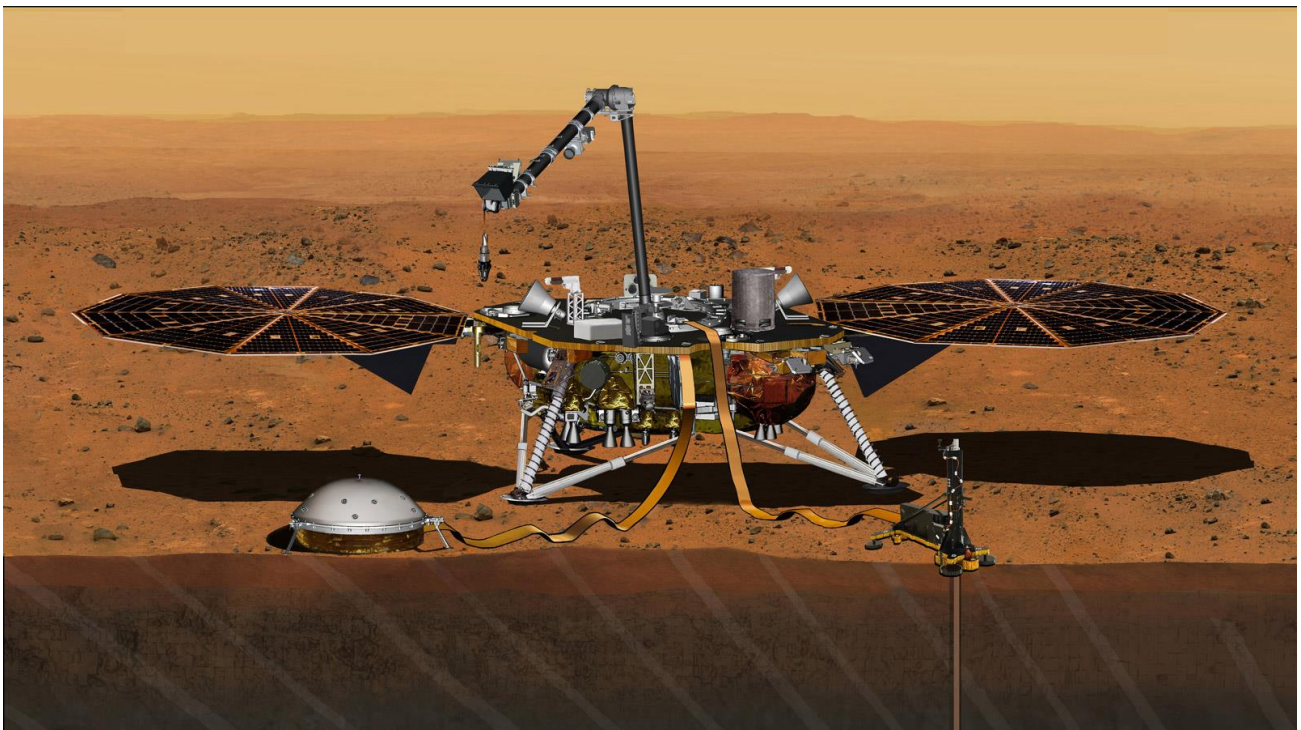
InSight
