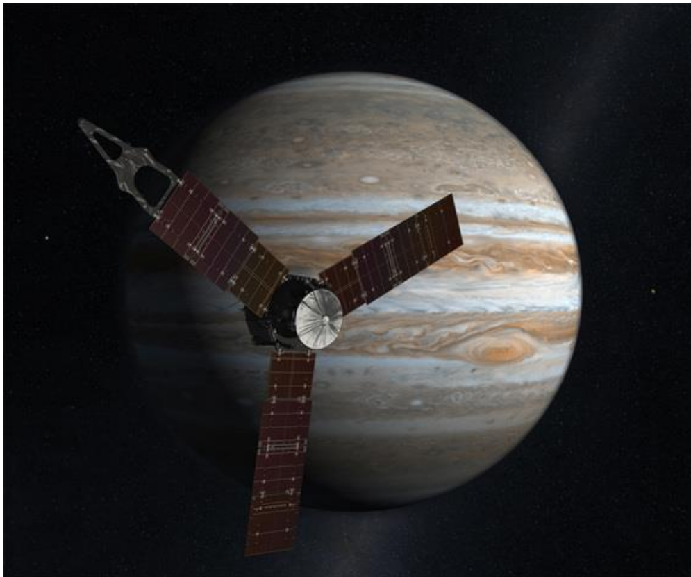
Juno Spacecraft
