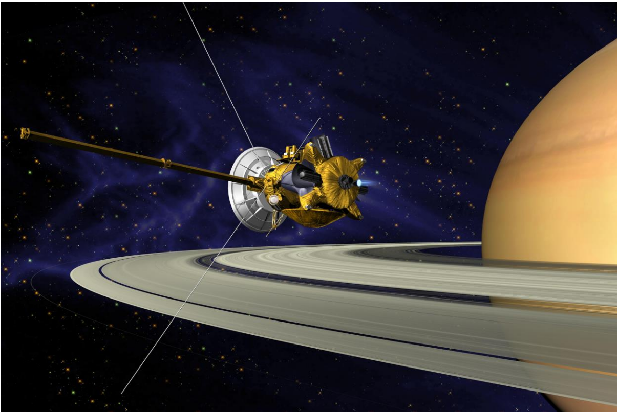
Cassini Spacecraft
