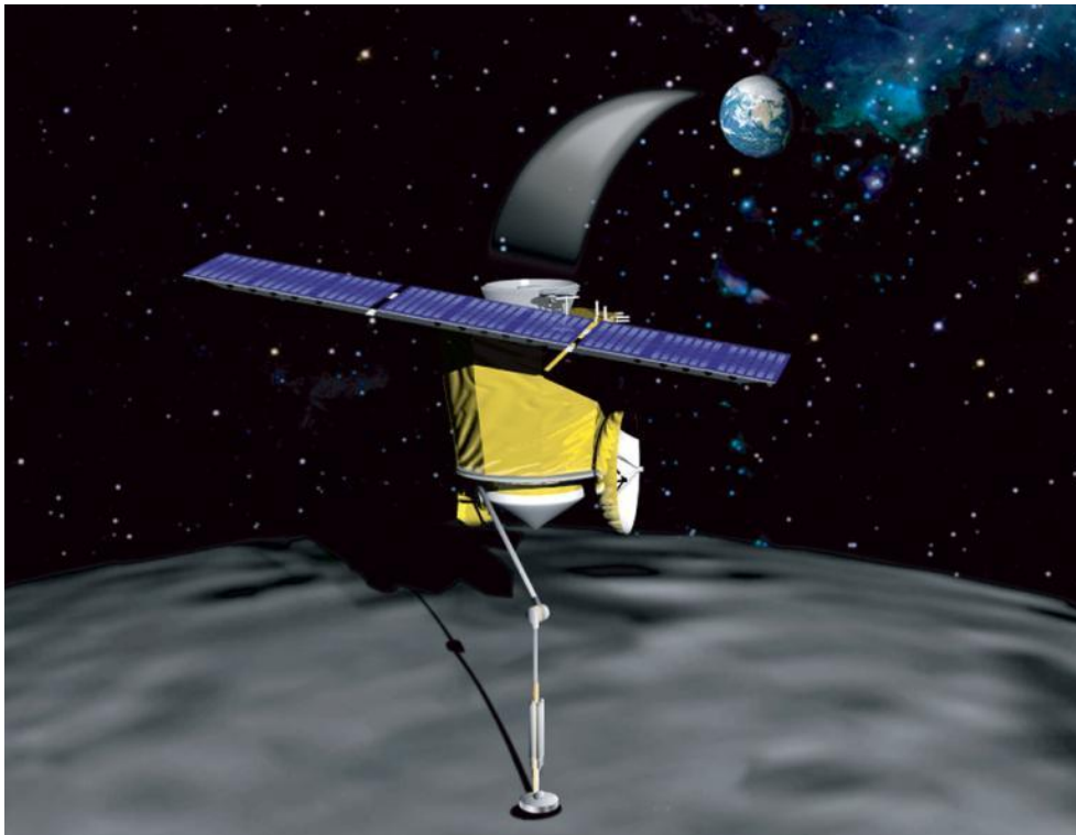
OSIRIS-REx Spacecraft
