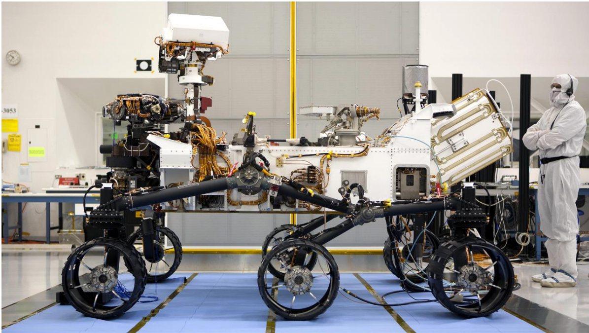
Curiosity Rover
