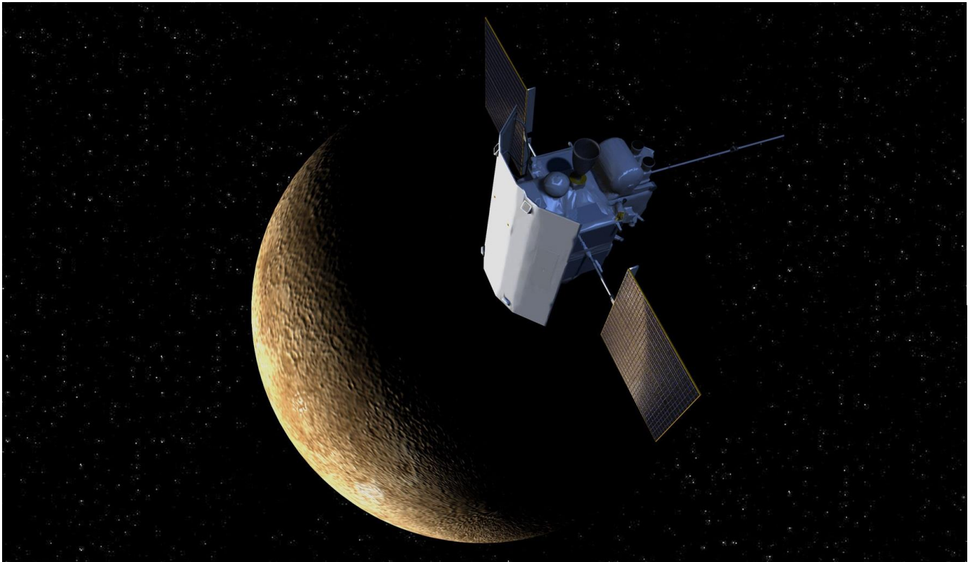
Messenger
