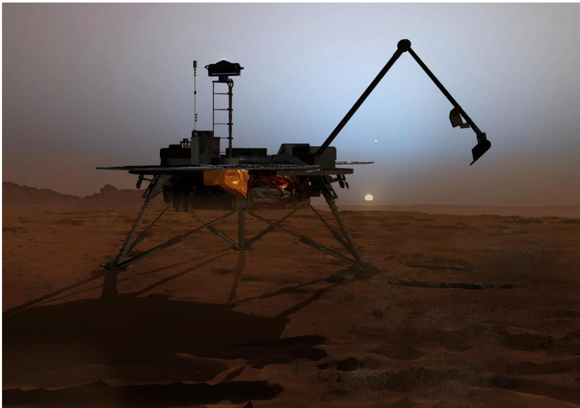
Phoenix Lander
